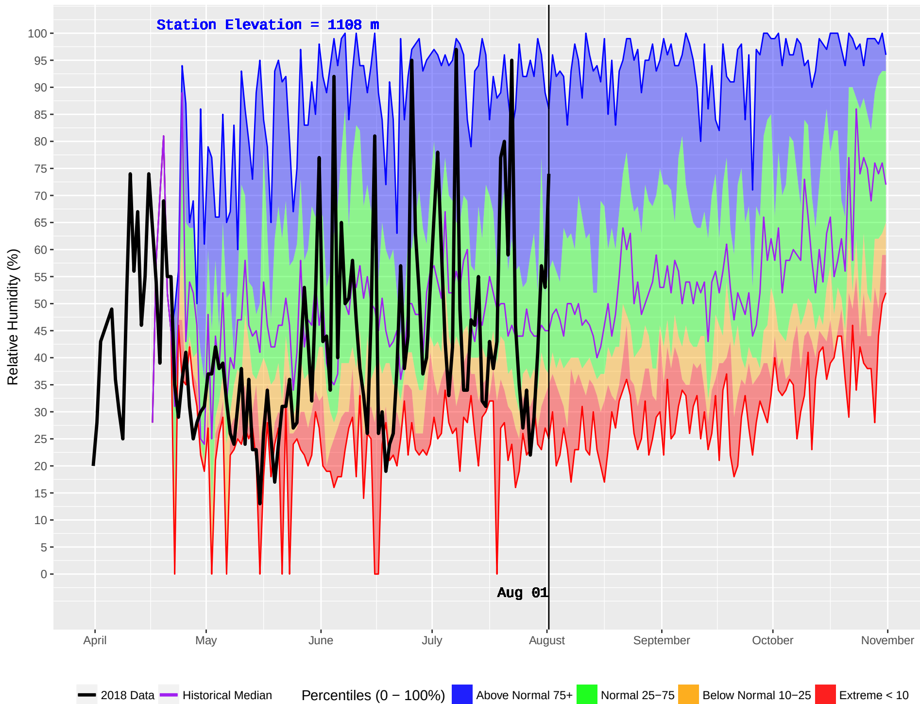
NABESHE (151) : Historical (1987–2016) and Current (2018) Daily Relative Humidity
